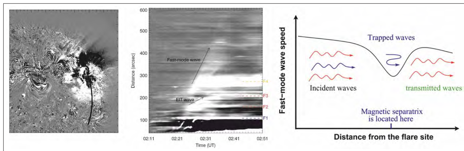
Fig 1: Left: SDO/AIA 193 Å difference image [02:11 UT, 11 May 2011] with a black line indicating the path for the time-distance diagram. Middle: Time-distance diagram showing two EUV wave components and stationary fronts [F1–F4]. Arrows highlight the fast MHD wave and the slower EIT wave [non-wave component]. Right: Schematic illustrating the physical process behind stationary front F4 [adapted from Chandra et al. 2016 [9]].
